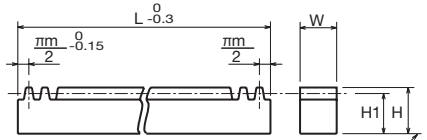
Gear-Cutting Reference Surface
