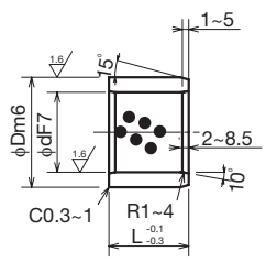
Oilless Bushing/Straight Type KPB Series
