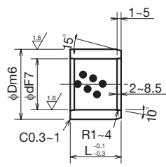
Oilless Bushing/Straight Type KPB Series
