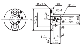
Oilless Bushing/Thrust Type (with Mounting Hole) KPS Series
