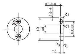
Oilless Bushing/Washer Type KPW Series
